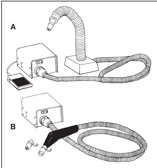
Figure 1. Desco Ion Python Air Nozzles A. Ion Python (Controller and Foot Switch) B. Hand Gun (Controller with Hose)
