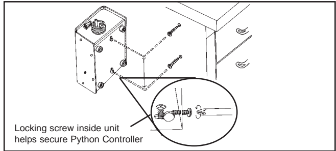
Figure 6. Installing controller to bench.
